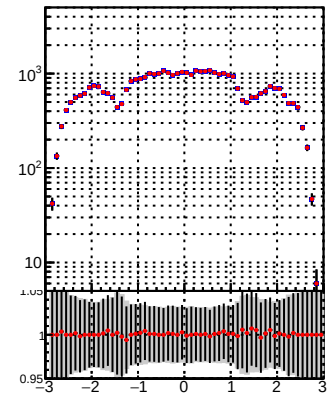
N of reco track vs \eta DQM_TT_mkFit-DQM_init_orig N of reco track vs \eta DQM_TT_mkFit-DQM_init_modi2
