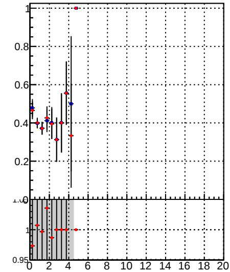
Fake rate vs. — DQM_TT_mkFit-DQM_init_orig — DQM_TT_mkFit-DQM_init_modi2
