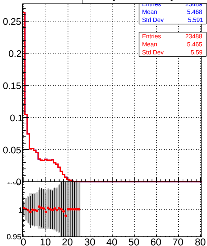
Legend: Grey bar: DQM_TT_mkFit-DQM_init_orig Red line with dots: DQM_TT_mkFit-DQM_init_modi2
