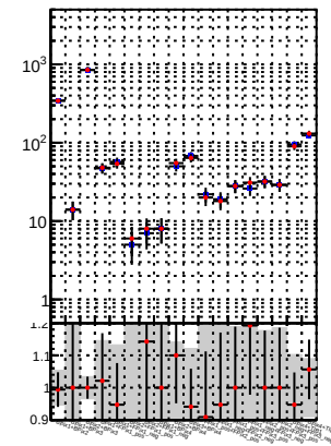
N of reco track vs. \chi^2 —•— mkFit-DQM_init_orig —•— mkFit-DQM_init_mod12
