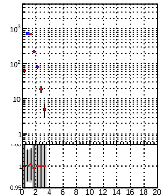
N of reco track vs. \chi^2 —•— mkFit-DQM_init_orig —•— mkFit-DQM_init_mod12
