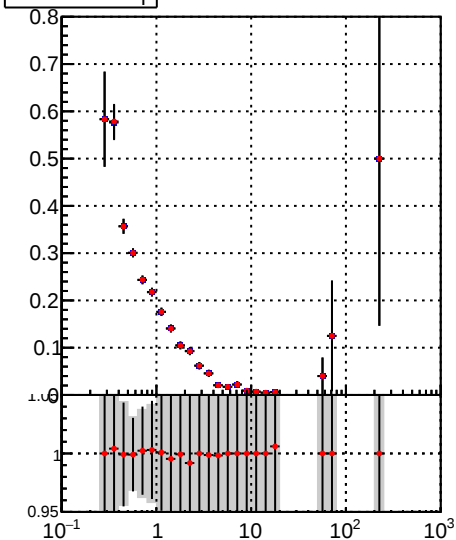
■ — ● DQM_TT_mkFit-DQM_init_orig — ● DQM_TT_mkFit-DQM_init_modi2
