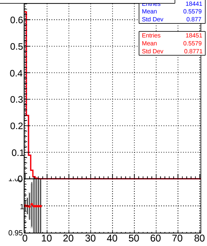
Legend: ■ DQM_TT_mkFit-DQM_init_orig ● DQM_TT_mkFit-DQM_init_modi2
