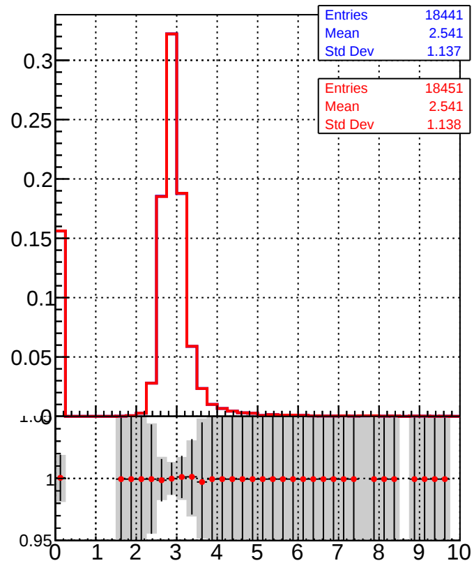
Legend: ■ DQM_TT_mkFit-DQM_init_orig ● DQM_TT_mkFit-DQM_init_modi2
