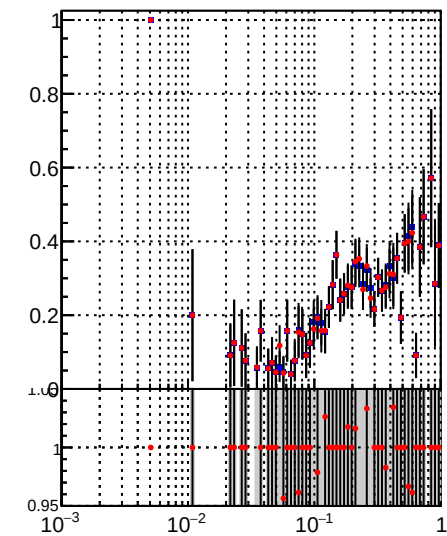
—•— DQM_TT_mkFit-DQM_init_orig —•— DQM_TT_mkFit-DQM_init_modi2
