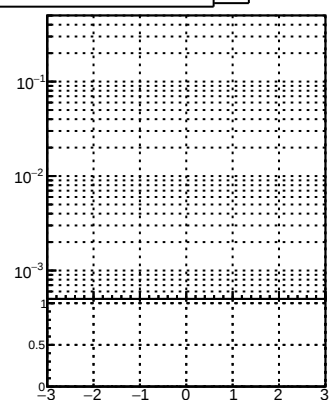
\eta
