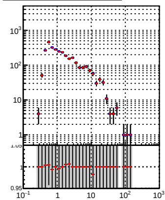
—●— DQM_TT_mkFit-DQM_init_orig —●— DQM_TT_mkFit-DQM_init_modi2
