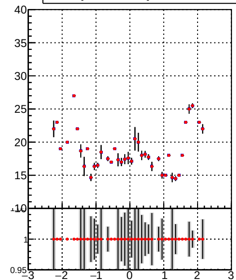
mean hit Legend: DQM_TT_mkFit-DQM_init_orig DQM_TT_mkFit-DQM_init_modi2
