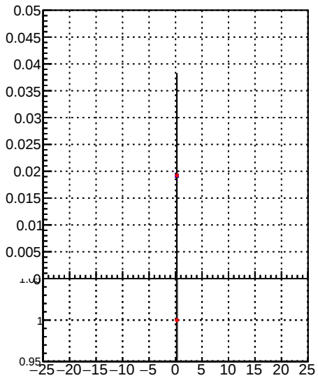
Fake rate vs d Legend: —•— DQM_TT_mkFit-DQM_init_orig —•— DQM_TT_mkFit-DQM_init_modi2
