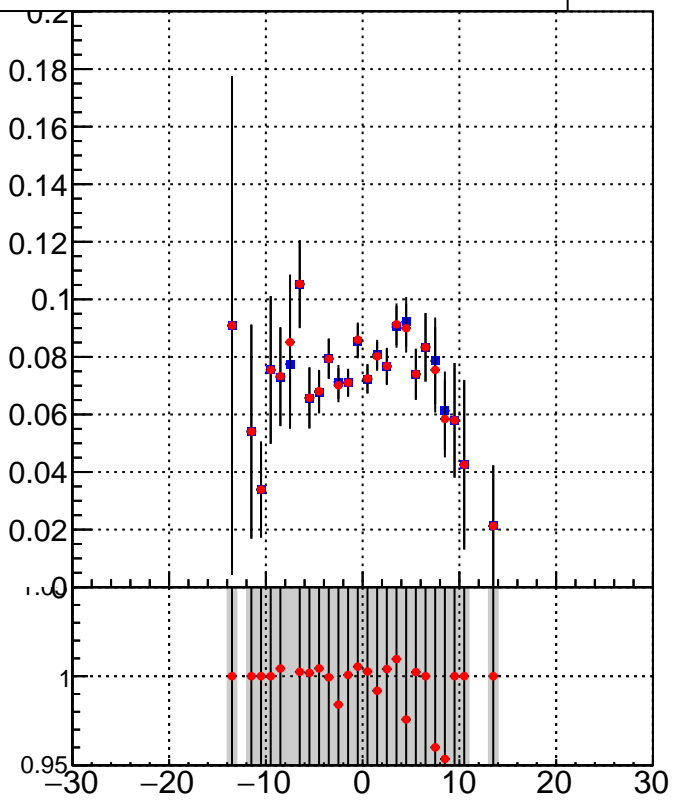
DQM_TT_mkFit-DQM_init_orig DQM_TT_mkFit-DQM_init_modi2
