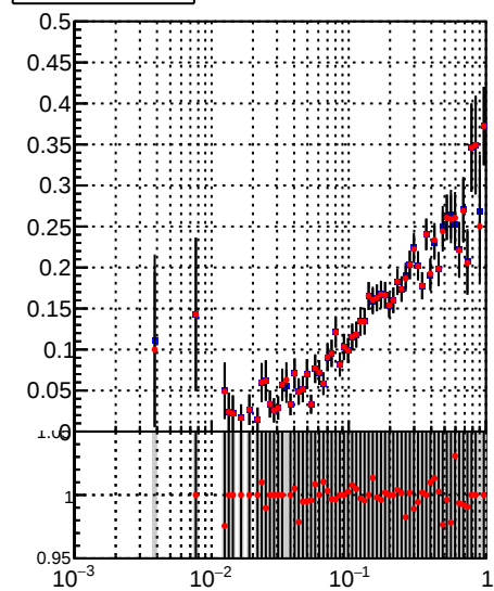
Pileup rate vs \sqrt{s}
