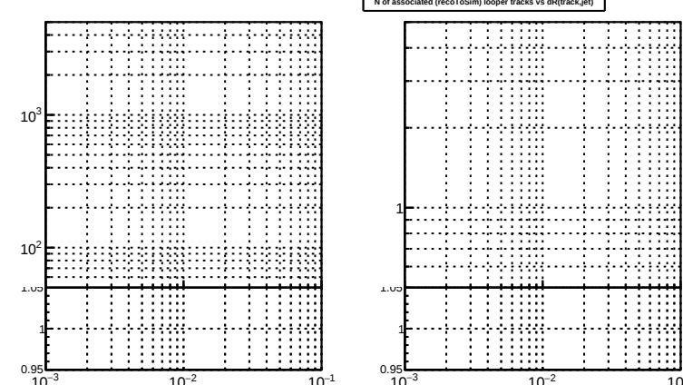
N of associated (recoToSim) looper tracks vs dR(track,jet)
