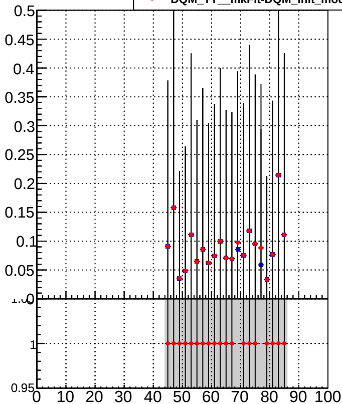
■ DQM_TT_mkFit-DQM_init_orig ● DQM_TT_mkFit-DQM_init_modi2
