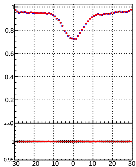
—•— DQM_TT_mkFit-DQM_init_orig —•— DQM_TT_mkFit-DQM_init_modi2
