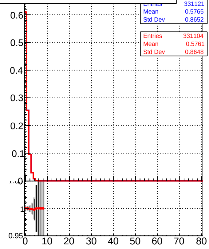
Legend: DQM_TT_mkFit-DQM_init_orig (grey histogram) DQM_TT_mkFit-DQM_init_modi2 (red histogram)
