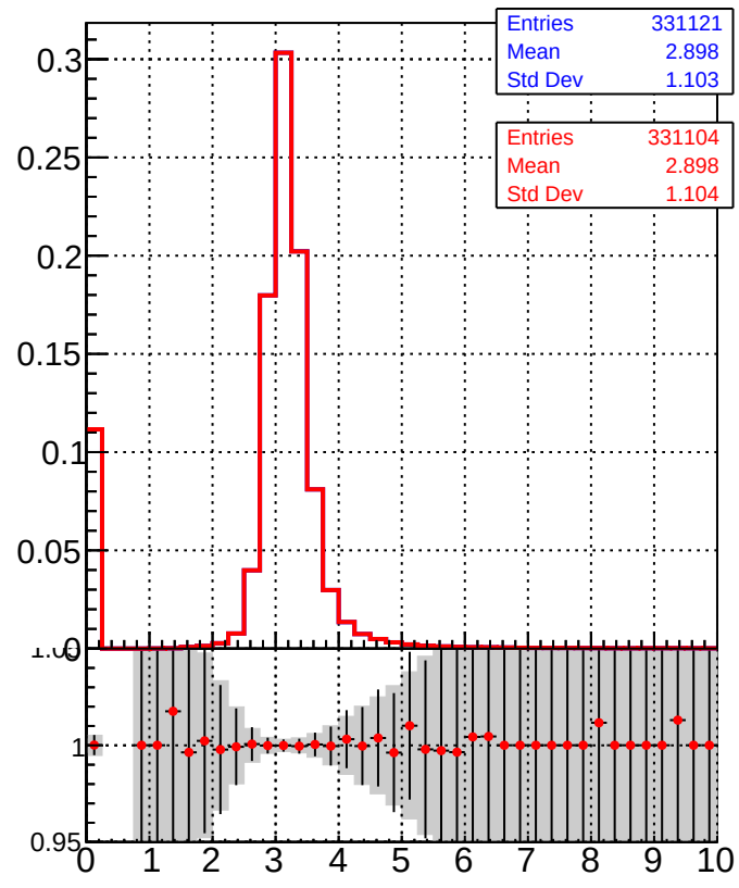
Legend: DQM_TT_mkFit-DQM_init_orig (grey histogram) DQM_TT_mkFit-DQM_init_modi2 (red histogram)
