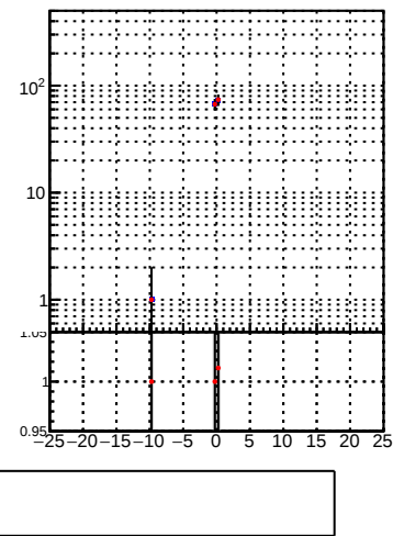
N of associated tracks (simToReco) vs dxy(PV)
