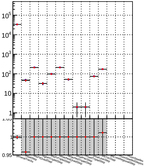
Number ● DQM_TT_mkFit-DQM_init_modi2
