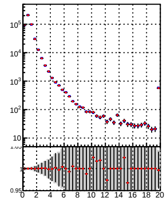
N of origi (recoToSim) tracks vs normalized \chi^2
