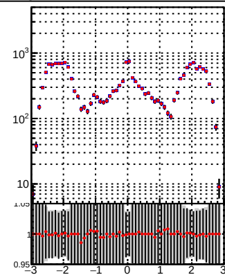
—•— DQM_TT_mkFit-DQM_init_orig —•— DQM_TT_mkFit-DQM_init_modi2
