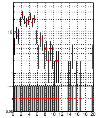
N of reco track vs. \chi^2 (Legend) DQM_TT mkFit-DQM_init_orig DQM_TT mkFit-DQM_init_modi2
