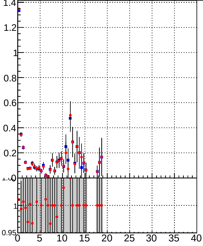
K_S^0 tracking fake rate vs p_T and \eta Legend: \blacksquare DQM_TT_mkFit-DQM_init_orig \bullet DQM_TT_mkFit-DQM_init_modi2
