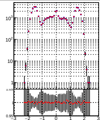
N of reco track vs \phi DQM_TT_mkFit-DQM_init_orig DQM_TT_mkFit-DQM_init_modi2
