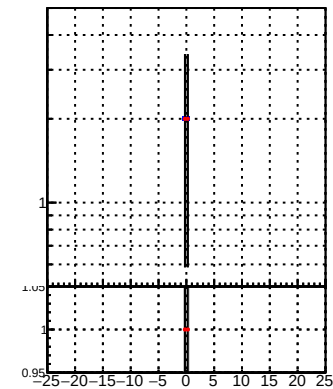
—•— DQM_TT_mkFit-DQM_init_orig —•— DQM_TT_mkFit-DQM_init_modi2
