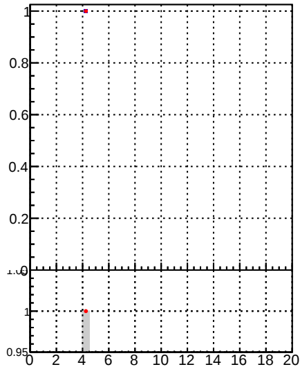
Fake rate vs. — \bullet DQM_TT_mkFit-DQM_init_orig — \bullet DQM_TT_mkFit-DQM_init_modi2
