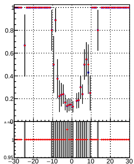
Fake rate vs d Legend: - DQM TT mkFit-DQM_init_orig (blue dots) - DQM TT mkFit-DQM_init_modi2 (red dots)
