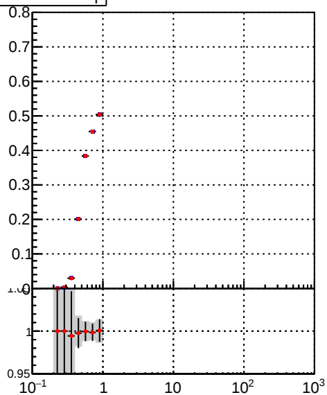
—■— DQM_TT_mkFit-DQM_init_orig —●— DQM_TT_mkFit-DQM_init_modi
