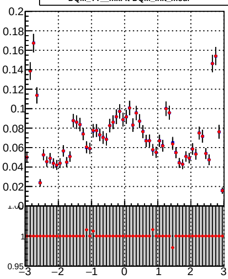
—■— DQM_TT_mkFit-DQM_init_orig —●— DQM_TT_mkFit-DQM_init_modi
