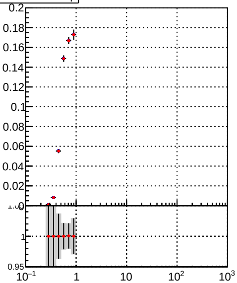
—■— DQM_TT_mkFit-DQM_init_orig —●— DQM_TT_mkFit-DQM_init_modi
