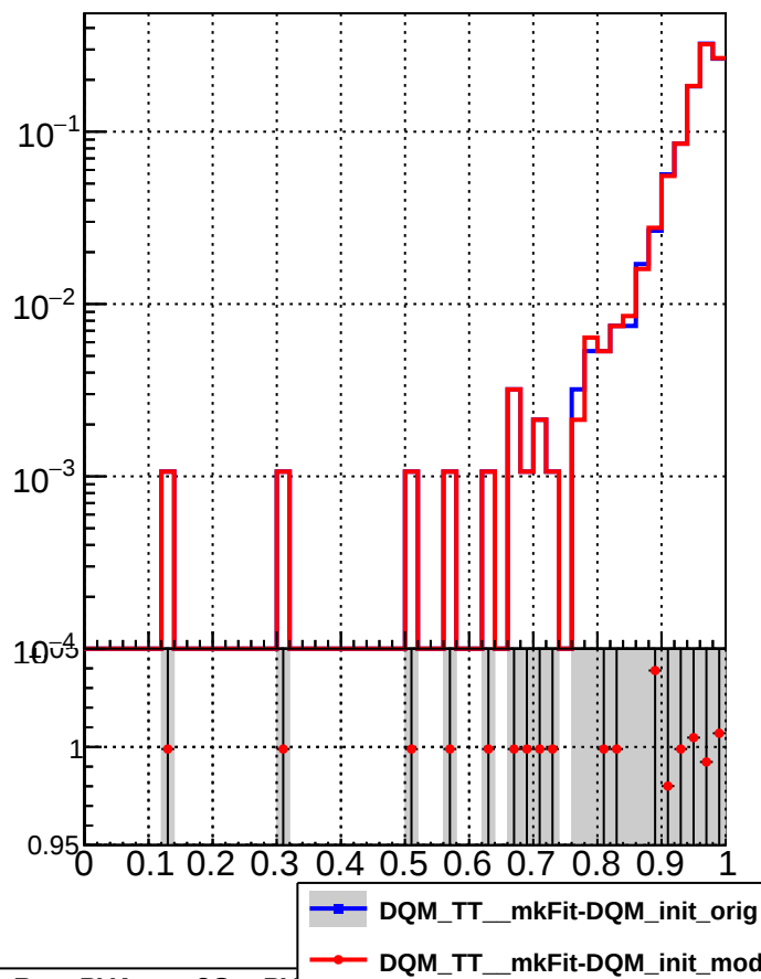
RecoPVAssoc2GenPVMatched_Missing
