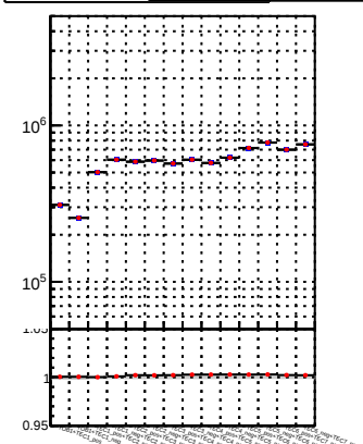
N of reco track vs. \chi^2 mkFit-DQM_init_orig mkFit-DQM_init_modi
