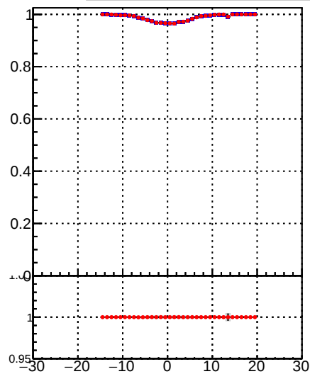
—•— DQM_TT_mkFit-DQM_init_orig —•— DQM_TT_mkFit-DQM_init_modi
