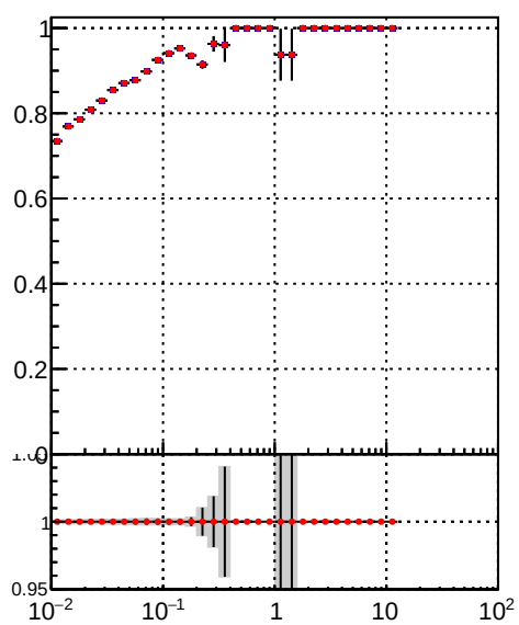
Efficiency vs. sim PV z Legend: DQM_TT_mkFit-DQM_init_orig DQM_TT_mkFit-DQM_init_modi
