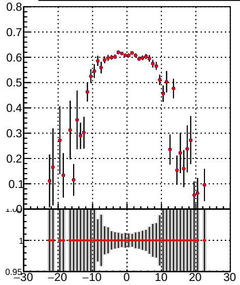
Efficiency vs. sim PV z Legend: DQM_TT_mkFit-DQM_init_orig DQM_TT_mkFit-DQM_init_modi
