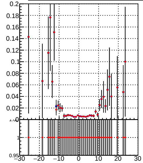
Efficiency vs vertpos — DQM_TT_mkFit-DQM_init_orig — DQM_TT_mkFit-DQM_init_modi
