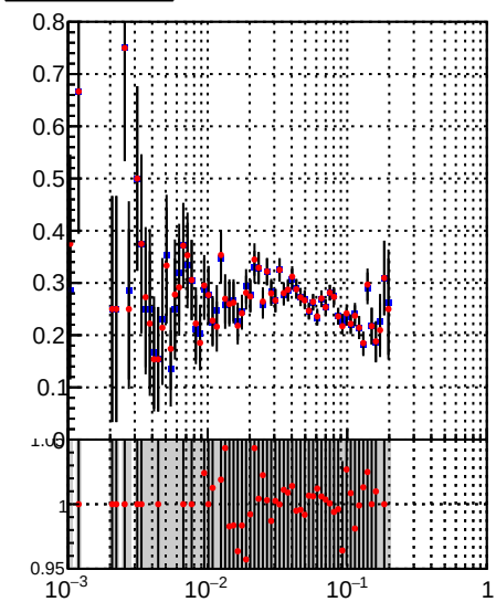
Fake rate vs \sqrt{s} DQM_TT_mkFit-DQM_init_orig DQM_TT_mkFit-DQM_init_modi
