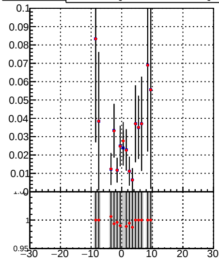
—•— DQM_TT_mkFit-DQM_init_orig —•— DQM_TT_mkFit-DQM_init_modi
