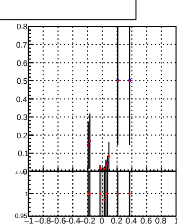
Pileup rate vs dxypv
