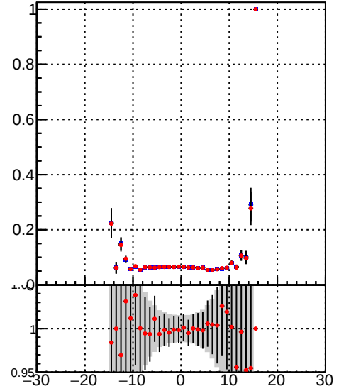
Efficiency vs. sim PV z Legend: DQM_TT_mkFit-DQM_init_orig (Blue line with error bars) DQM_TT_mkFit-DQM_init_modi (Red line with error bars)
