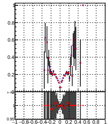
—●— DQM_TT_mkFit-DQM_init_orig —●— DQM_TT_mkFit-DQM_init_modi
