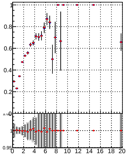
Fake rate vs. \text{DQM\_TT\_mkFit-DQM\_init\_orig} \text{DQM\_TT\_mkFit-DQM\_init\_modi}
