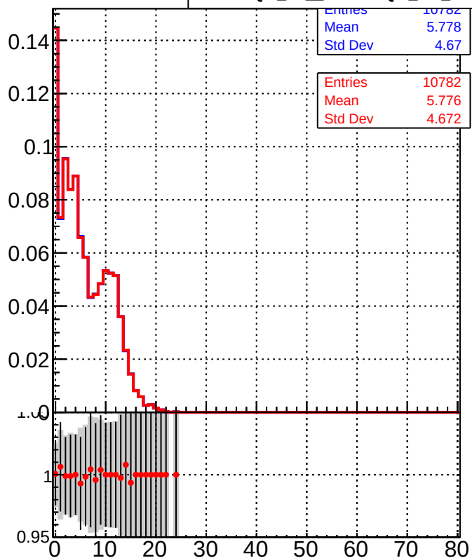
—■— DQM_TT_mkFit-DQM_init_orig —●— DQM_TT_mkFit-DQM_init_modi
