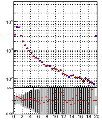
Legend: - Blue line with circles: DQM TT mkFit-DQM_init_orig - Red line with circles: DQM TT mkFit-DQM_init_mod - Grey shaded area: verBet
