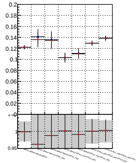
Fake rate vs. \text{DQM\_TT\_mkFit-DQM\_init\_orig} \text{DQM\_TT\_mkFit-DQM\_init\_modi}
