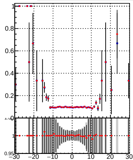
—•— DQM_TT_mkFit-DQM_init_orig —•— DQM_TT_mkFit-DQM_init_modi
