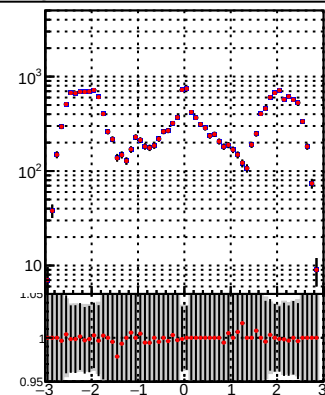
—●— DQM_TT_mkFit-DQM_init_orig —●— DQM_TT_mkFit-DQM_init_modi
