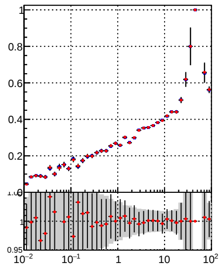
—●— DQM_TT_mkFit-DQM_init_orig —●— DQM_TT_mkFit-DQM_init_modi
