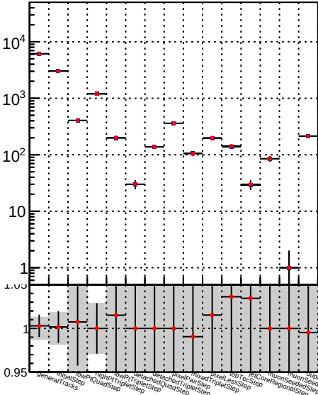
Number —●— DQM_TT_mkFit-DQM_init_modi
