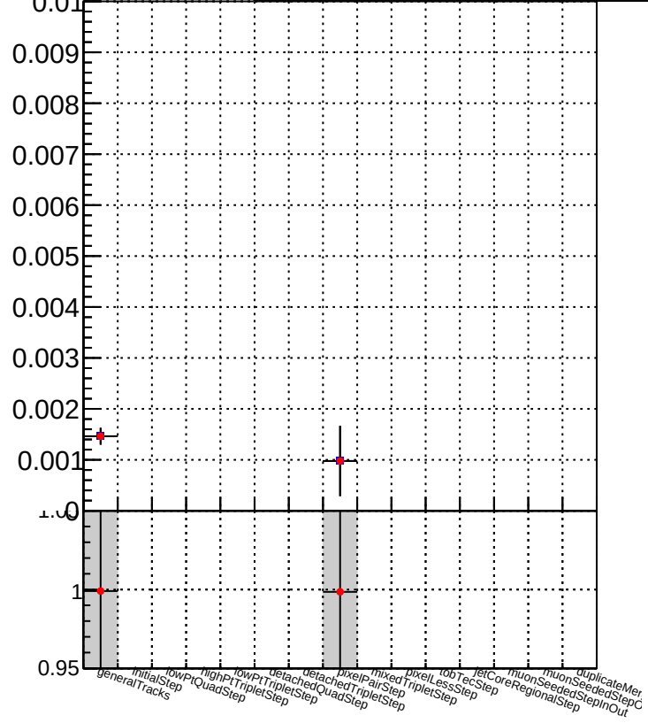
Duplicates rate vs collection Legend: ■ DQM_TT_mkFit-DQM_init_orig ● DQM_TT_mkFit-DQM_init_modi
