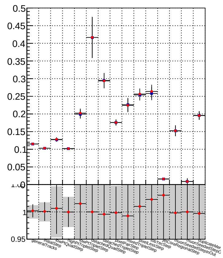
Duplicates rate vs collection Legend: ■ DQM_TT_mkFit-DQM_init_orig ● DQM_TT_mkFit-DQM_init_modi
