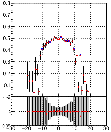
Efficiency vs. sim PV z Legend: DQM_TT_mkFit-DQM_init_orig (grey histogram) DQM_TT_mkFit-DQM_init_modi (red points with error bars)
