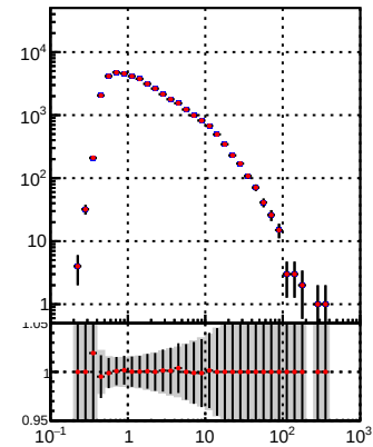
—●— DQM_TT_mkFit-DQM_init_orig —●— DQM_TT_mkFit-DQM_init_modi
