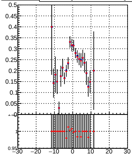
Fake rate vs v Legend: DQM_TT_mkFit-DQM_init_orig DQM_TT_mkFit-DQM_init_modi
